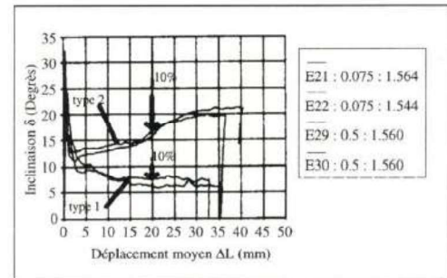
Figure 6 : Courbes \delta = f(DL) .
