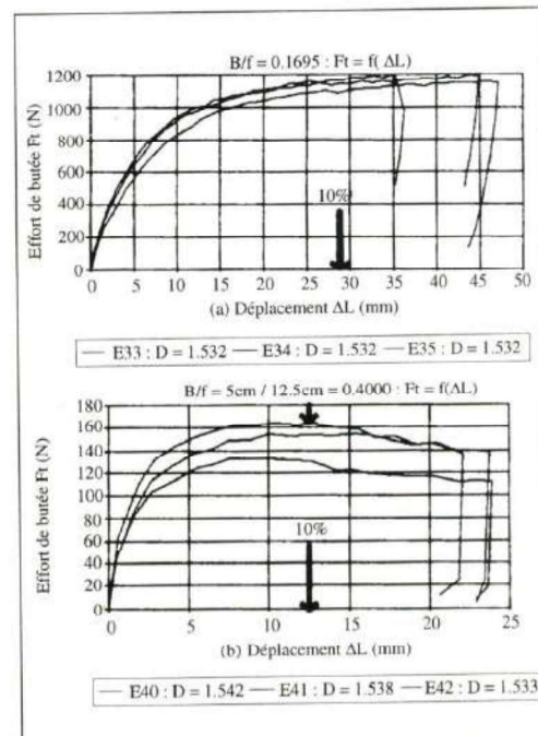
Figure 3 : Courbes F_t = f(\Delta L) .
